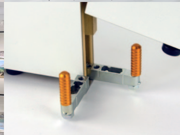
G40 Exzenterverbinder G40 off-center Connector
